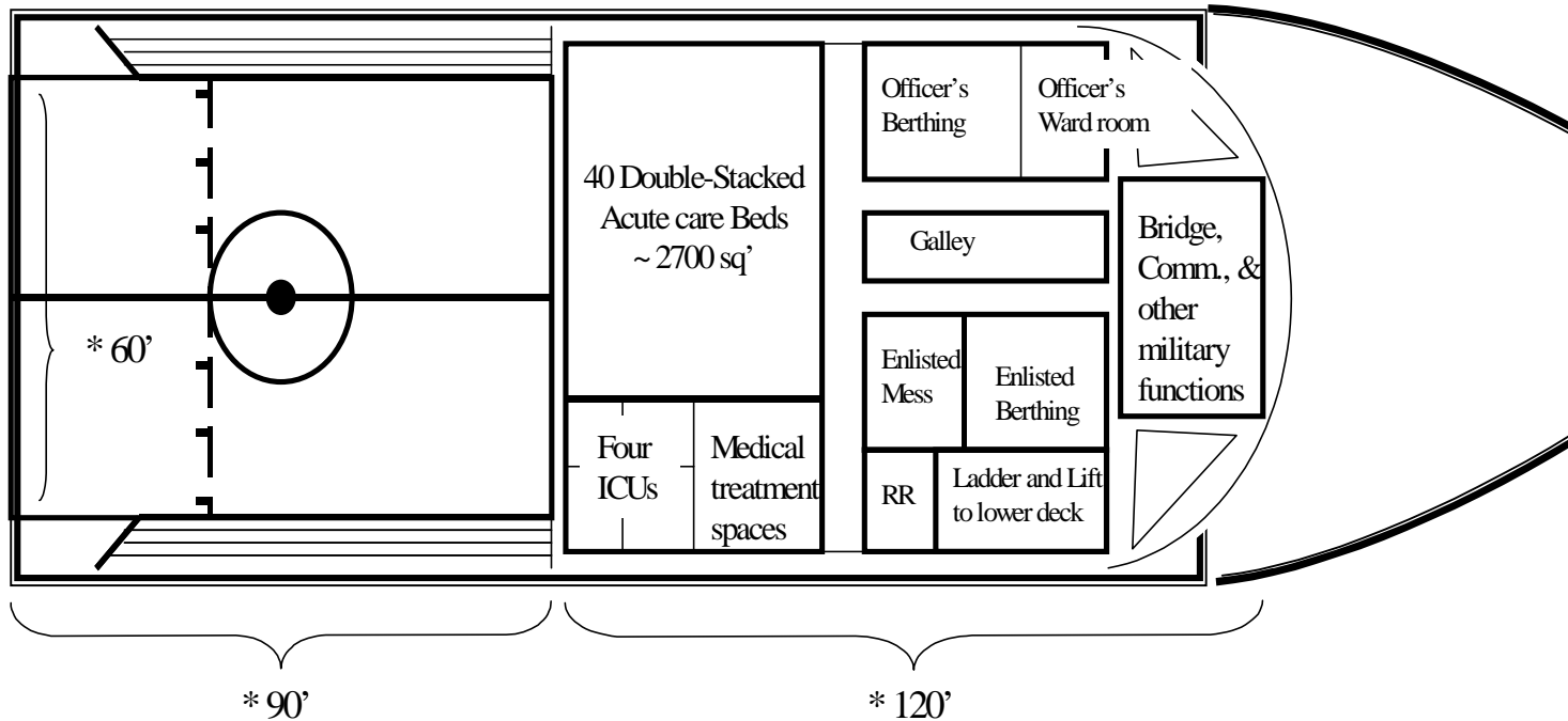
Figure 10. HSV-IX high-speed catamaran upper deck—notional limited medical ambulance and ship’s functions
