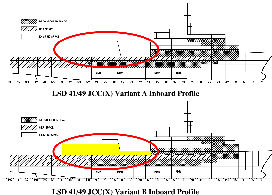
Figure 18. LSD 41/49 JCC(X) variants
