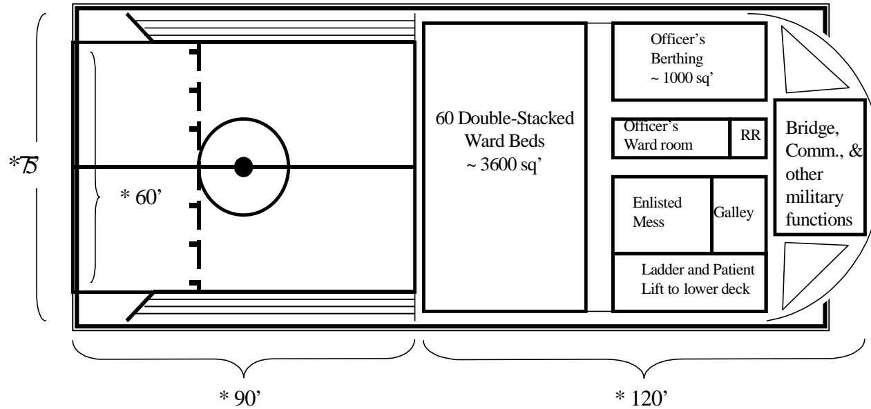
Figure 8. HSV-IX high-speed catamaran upper deck—notional medical ward and ship's functions
